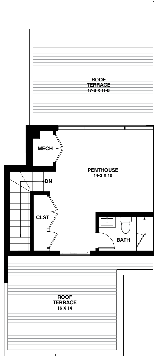
Roof Terrace
