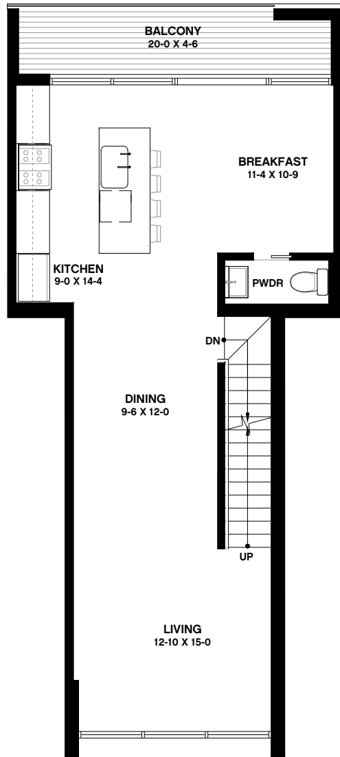
Second Floor
