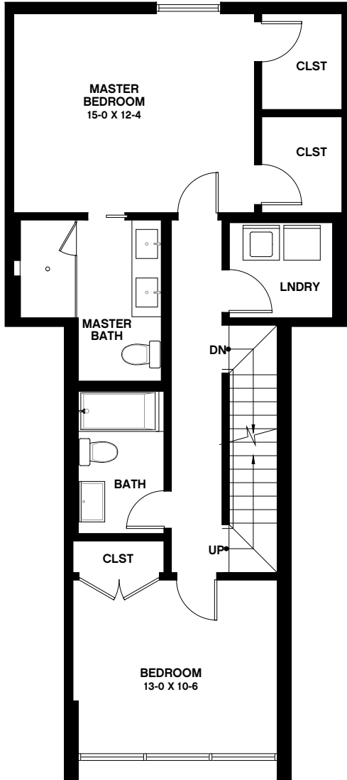
Third Floor
